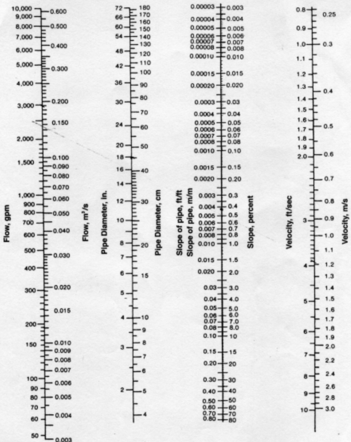
Figure 4-22 Nomograph for Manning formula in English and SI metric units for circular pipes flowing full based on n = 0.013 . (Courtesy of U.S. Pipe & Foundry Co.)
