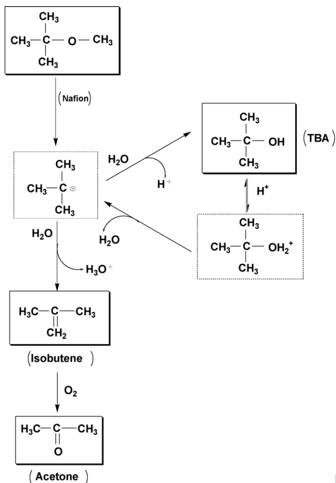
Fig. 2. A scheme of the reaction pathways for the transformation of MTBE with Nafion SAC-13.
