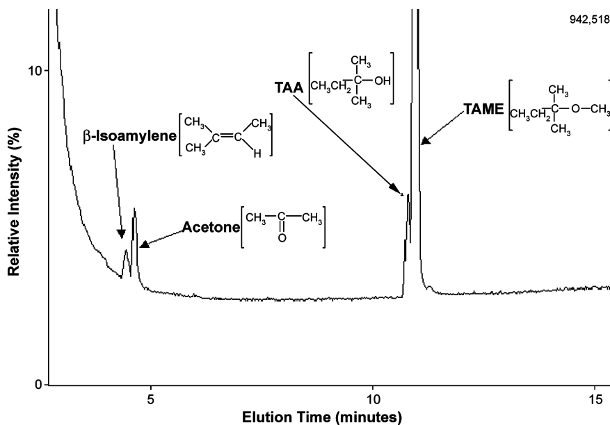
Fig. 3. A GC/MS chromatogram of TAME and products formed after a 12-h contact time.
