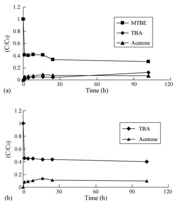
Fig. 1. (a) Transformation of MTBE over Nafion SAC-13. (b) Transformation of TBA over Nafion SAC-13. Initial concentrations of MTBE and TBA were 50 and 40 mg/l, respectively. Nafion loading was 4 g/50 ml.
