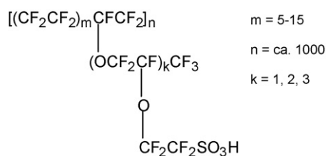
Scheme 1. Chemical structure of Nafion.
