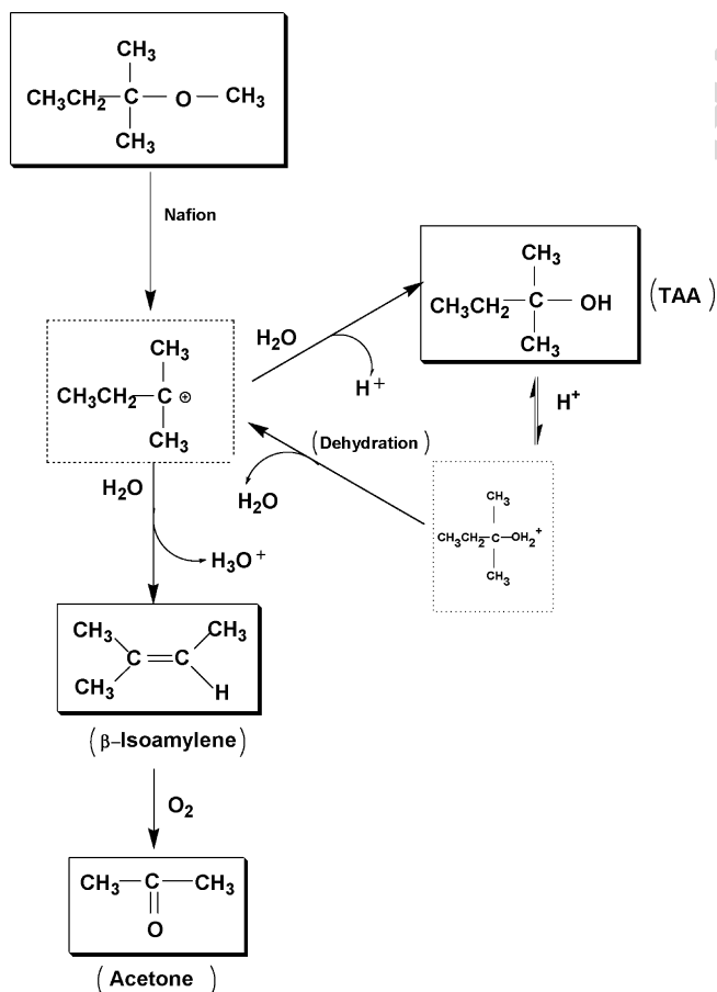
Fig. 4. A proposed reaction scheme for acid-catalyzed destruction of TAME over Nafion SAC-13.
