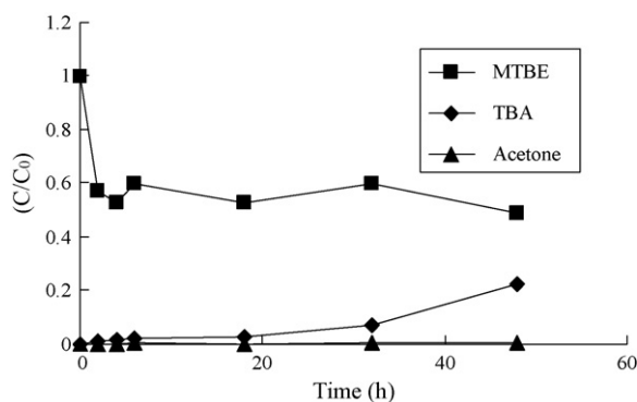
Fig. 5. Transformation of MTBE with Nafion SAC-13 in a N_2 -purged solution. Initial concentrations of MTBE was 40 mg/l. Nafion loading was 4 g/50 ml.
